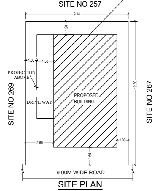
SITE PLAN
